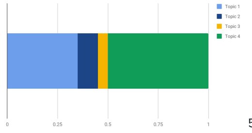
Topic distribution
