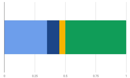
Topic distribution
